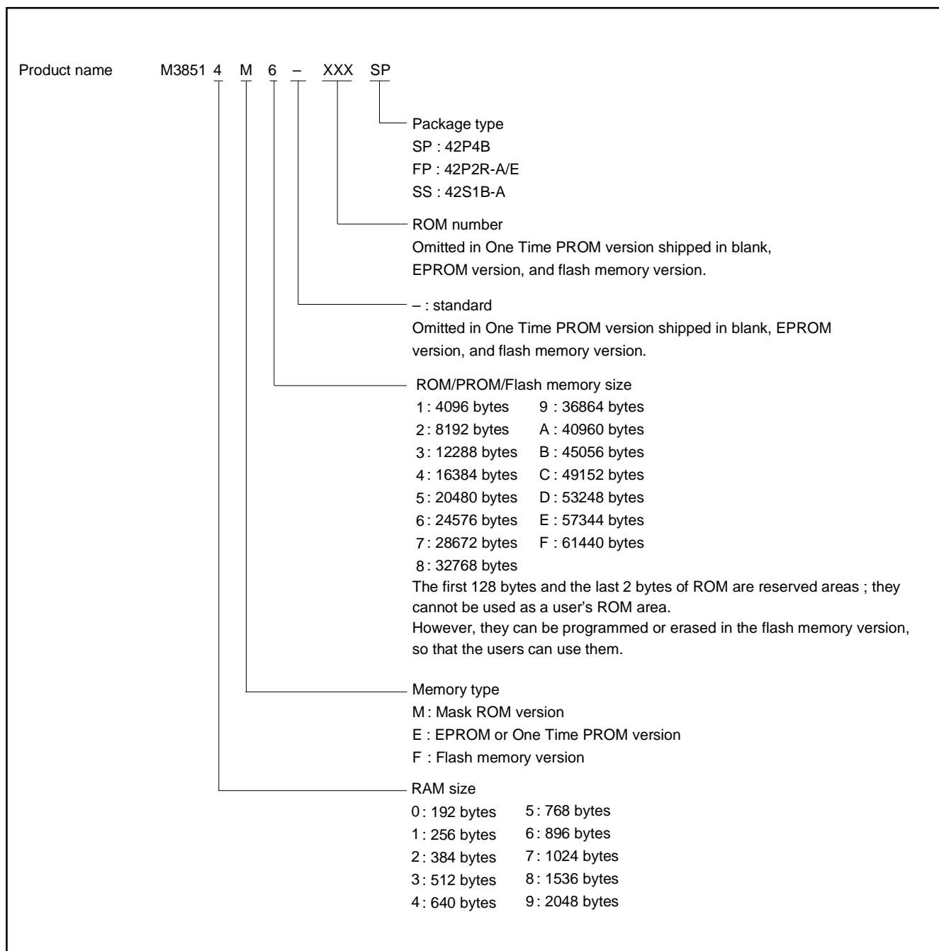
Fig. 3 Part numbering
